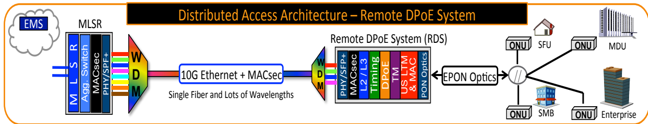
Figure 18 – DAA – Remote DPoE System (RDS)
