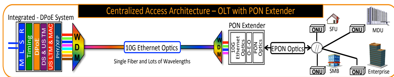
Figure 11 – CAA – OLT with PON Extender
