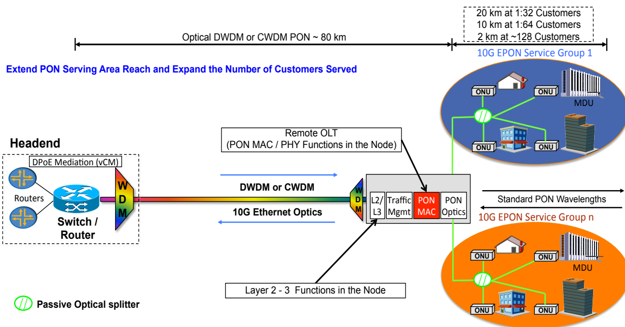
Figure 3 – High-Level – DAA - Remote OLT Network Architecture
