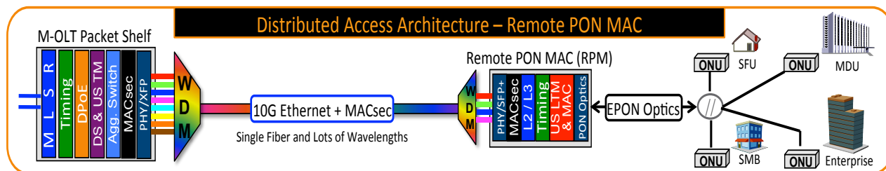
Figure 16 – DAA – Remote PON MAC (RPM)
