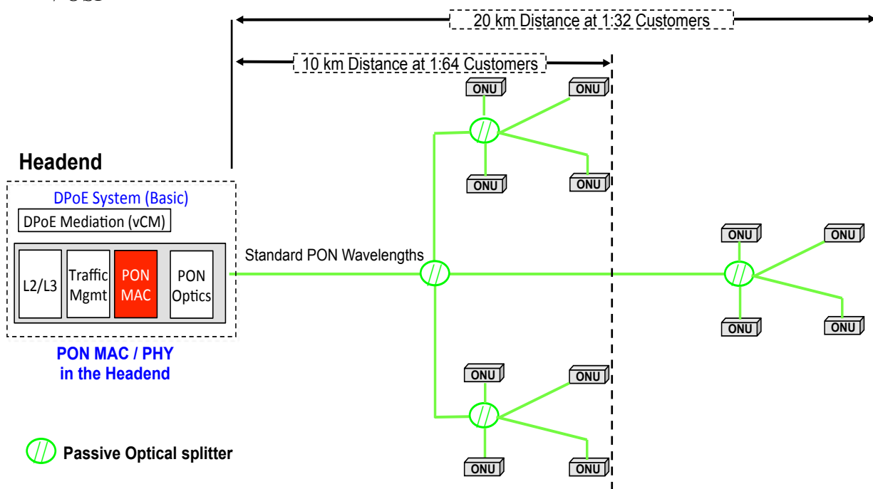
Figure 1 – High-Level – CAA DPoE System
