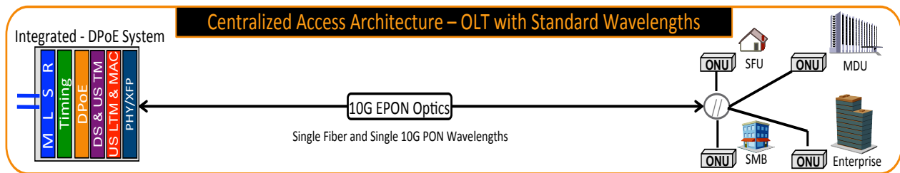
Figure 9 – CAA – OLT with Standard Wavelengths
