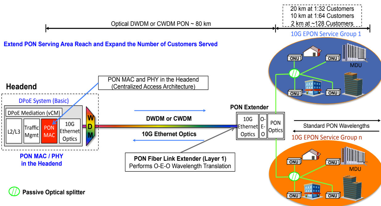
Figure 2 – High-Level – CAA PON Extender Network Architecture
