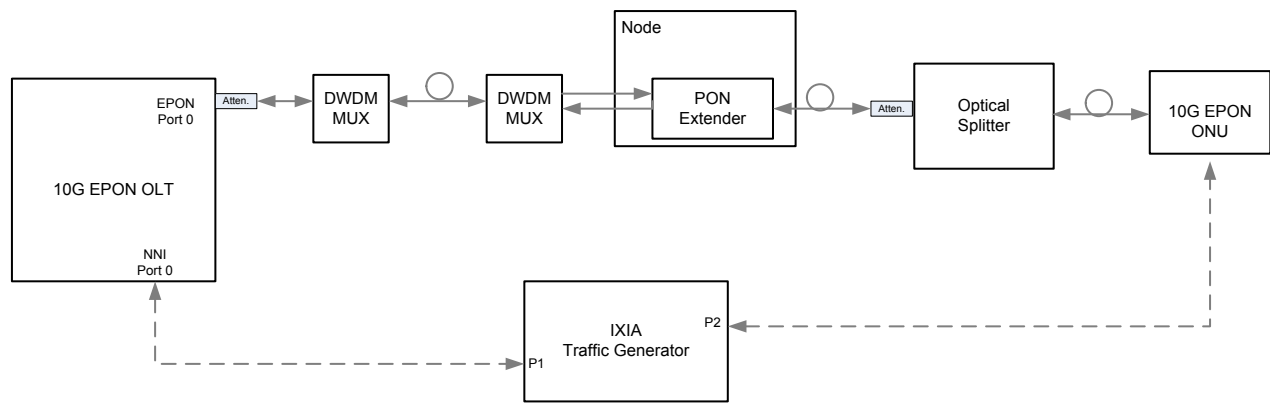
Figure 12 – Top: CAA – OLT with Standard Wavelengths Bottom: CAA – OLT with PON Extender
