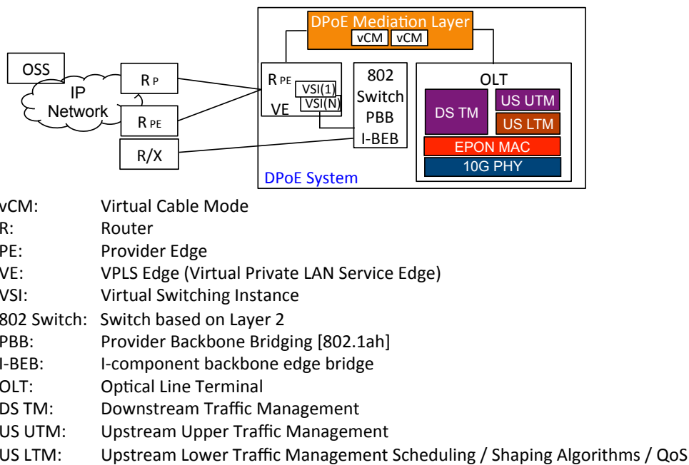
Figure 5 – OLT and DPoE Mediation Layer Subsystems
