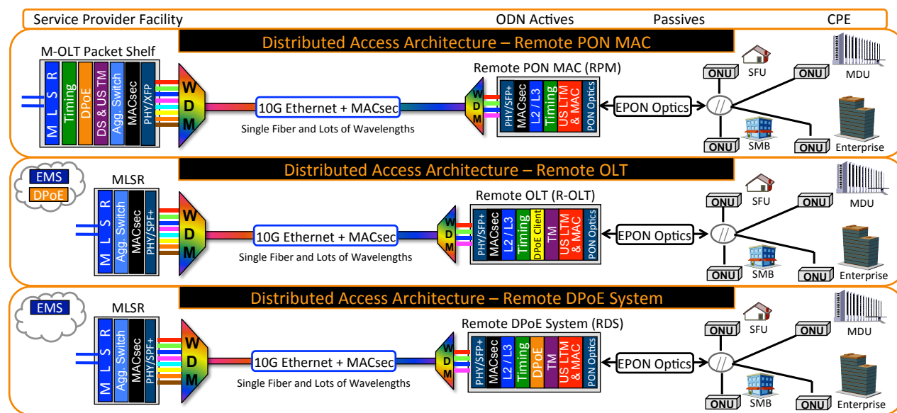
Figure 8 – Distributed Access Architecture (DAA) for PON Options
