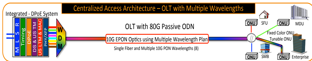
Figure 10 – CAA – OLT with Multiple Wavelengths
