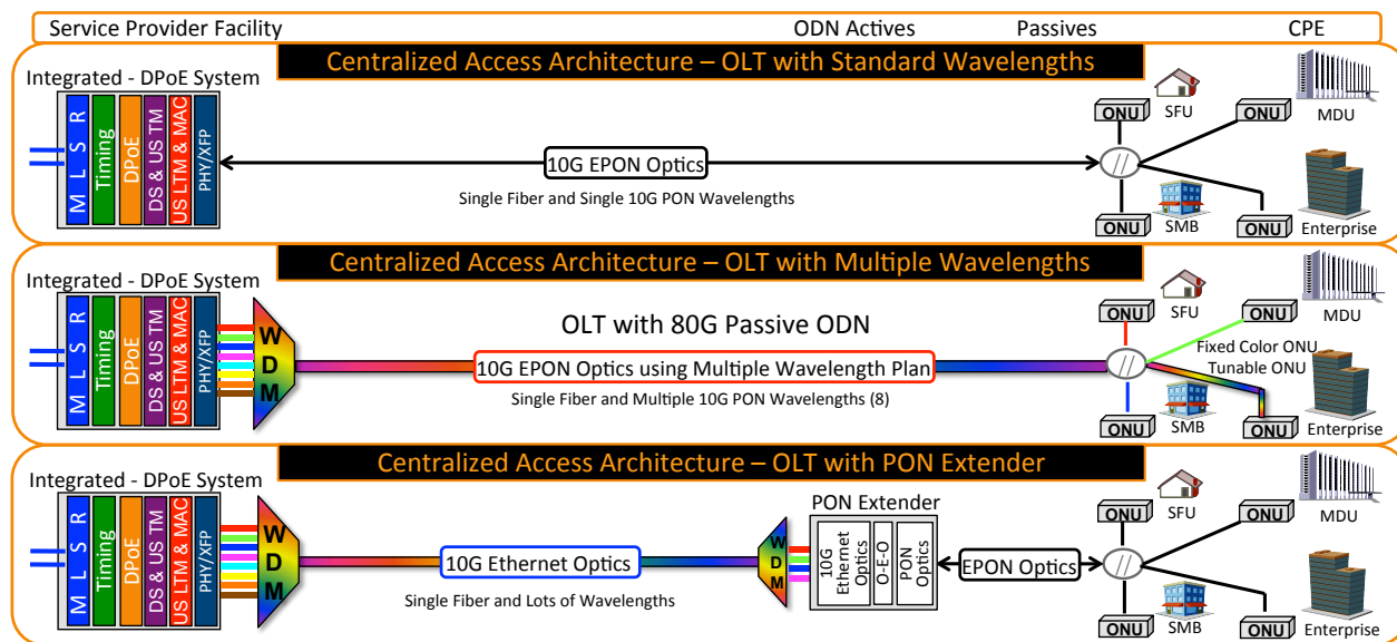
Figure 7 – Centralized Access Architecture (CAA) for PON Options
