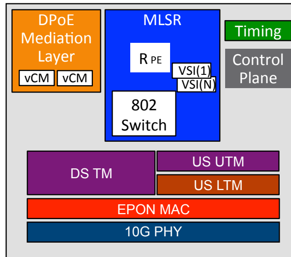
Figure 6 – Detailed Illustration of the DPoE Sub System Functions
