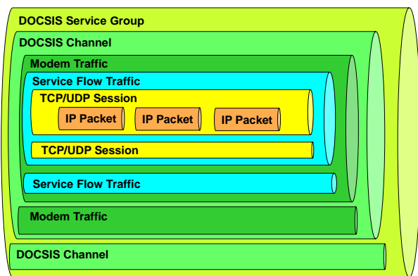
Fig. 2- Traffic Hierarchy
