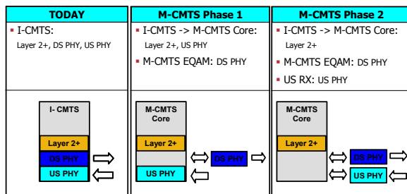
Figure 4. M-CMTS Migration Option A
